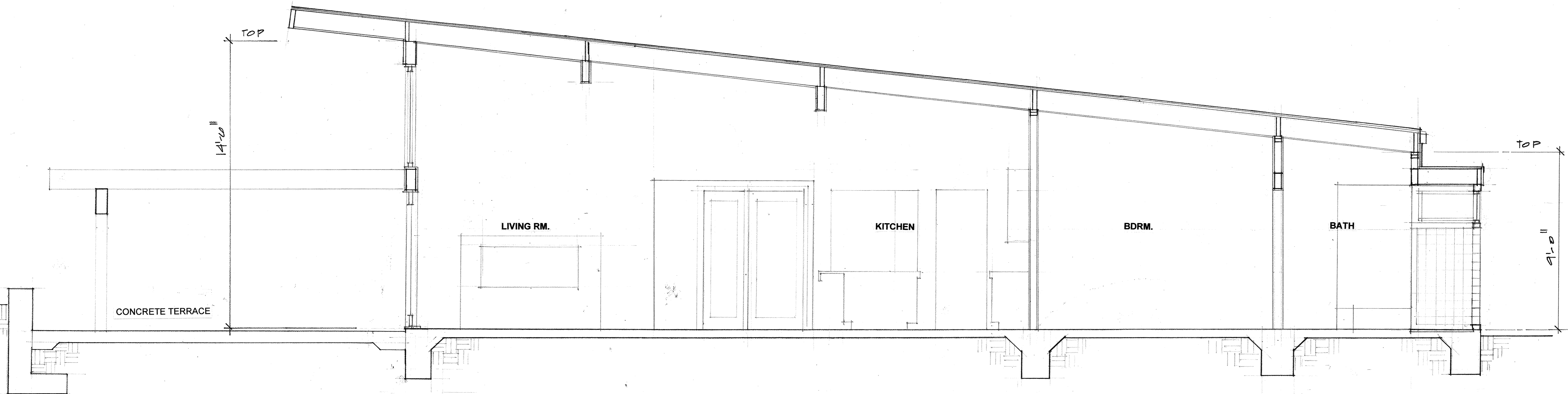
B-B BUILDING SECTION SCALE: 3/8"=1'-0"
