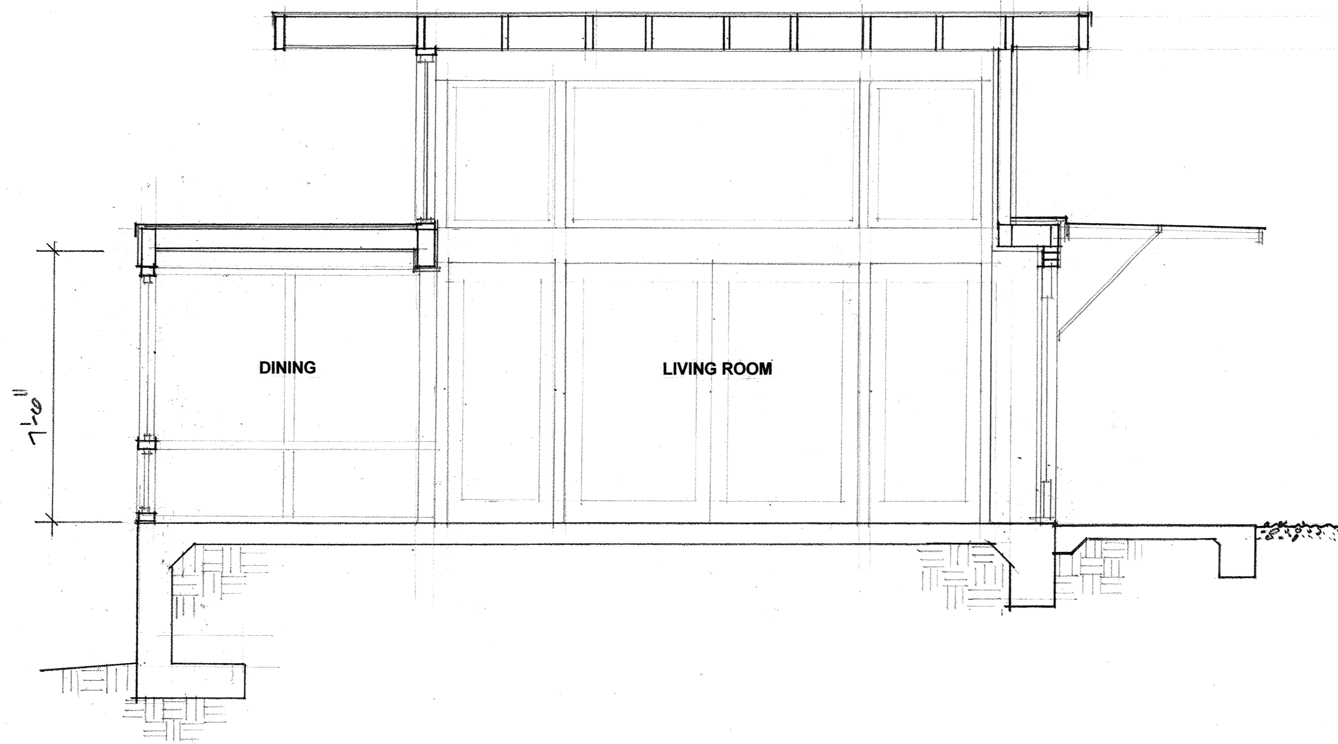
A-A BUILDING SECTION SCALE: 3/8"=1'-0"
